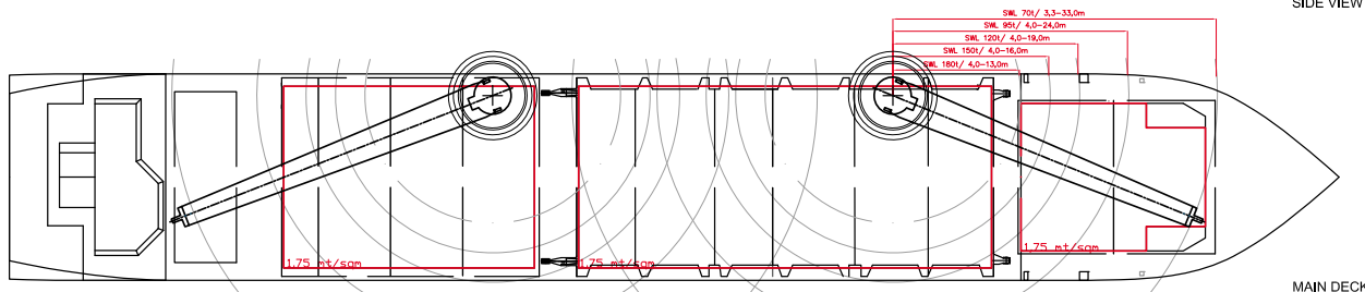
MAIN DECK
