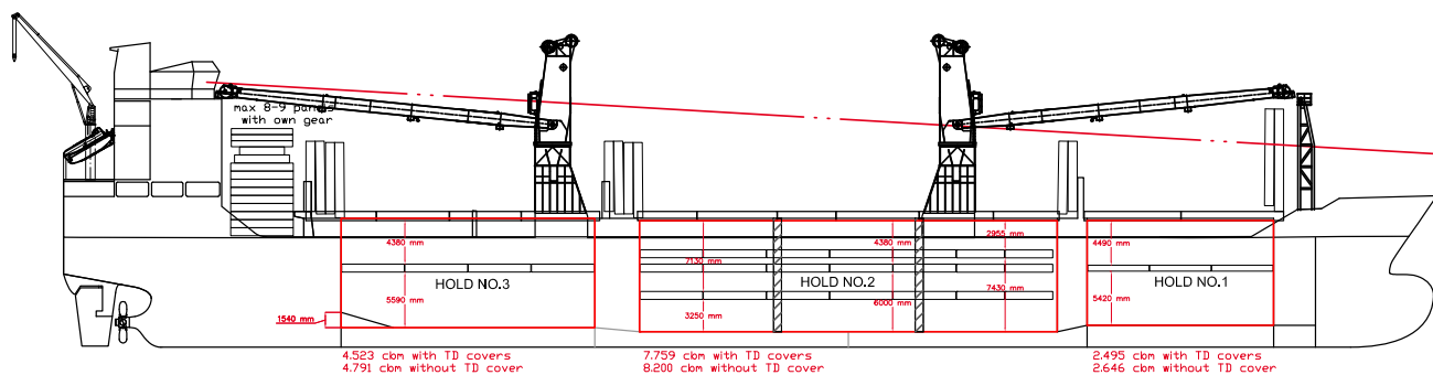
SIDE VIEW
